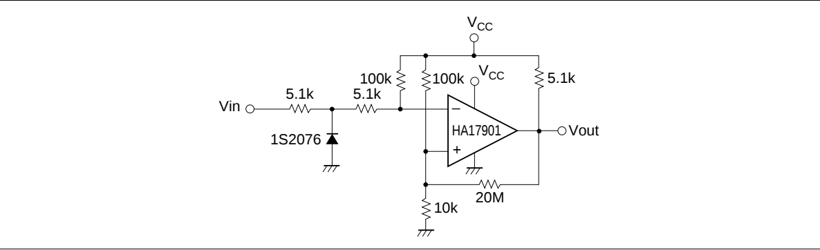
Figure 11 Zero-Cross Detector
